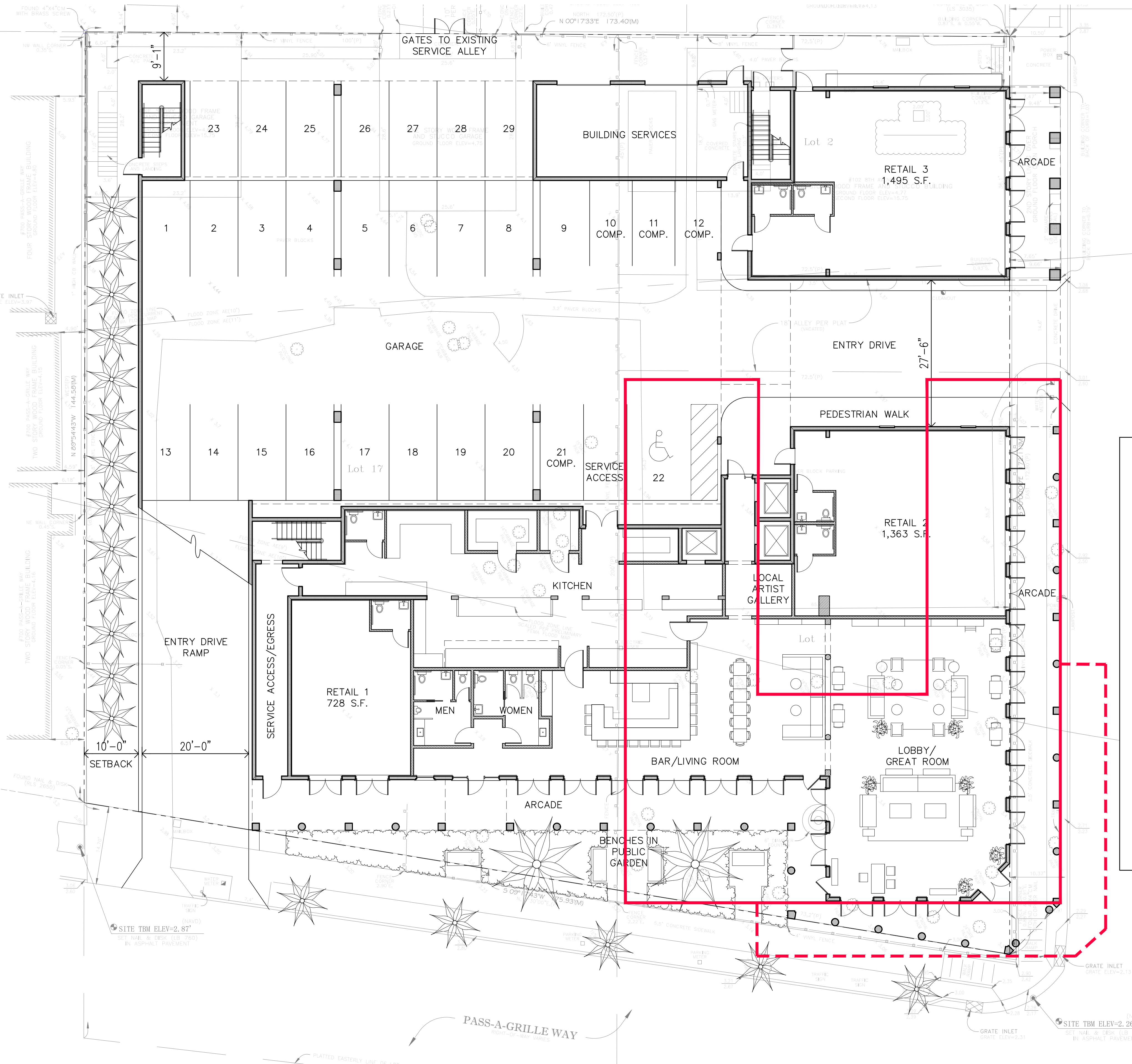
GROUND FLOOR PLAN/SITE PLAN
