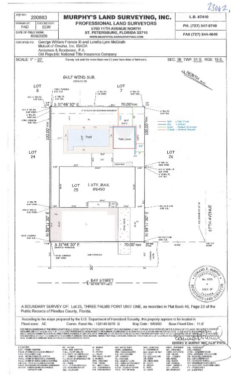
Figure 5: Survey with proposed structure (N.T.S.)
